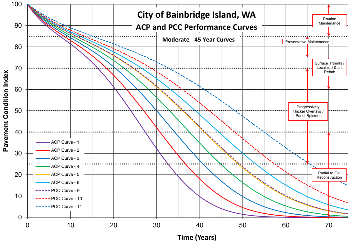
Figure 17 - Performance Curves
